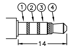
RECOMMENDED ϕ3.5 MATING PLUG
